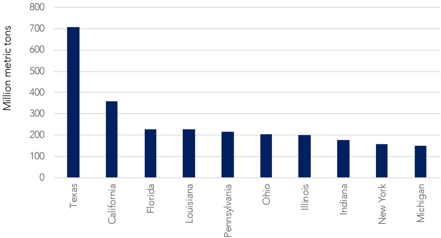
CO 2 emissions by states
